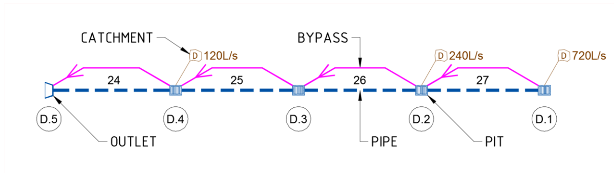
Diagram 1 – Network Configuration
